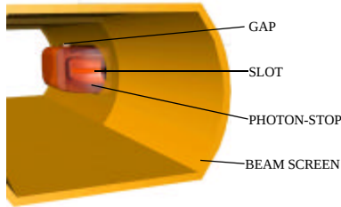
Figure 7: Sketch of the proposed VLHC-2 photon-stop.
