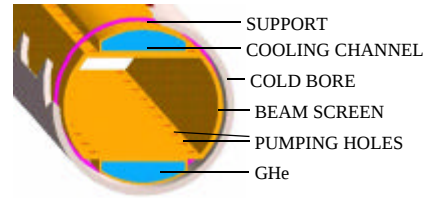
Figure 4: The proposed VLHC-2 beam-screen assembly.
