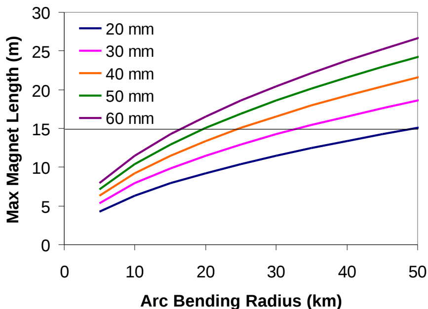
Figure 6: Maximum magnet length compatible with photon-stops versus arc bending radius, for the “N-2 scheme”.
