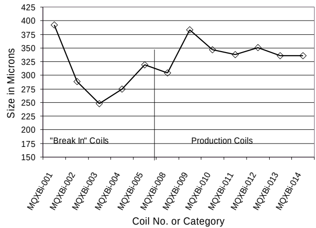
Figure 7. Average coil size relative to a steel master for long inner coils fabricated to date. Break In coils were made each made from different remnants of cable from the model magnet program.
