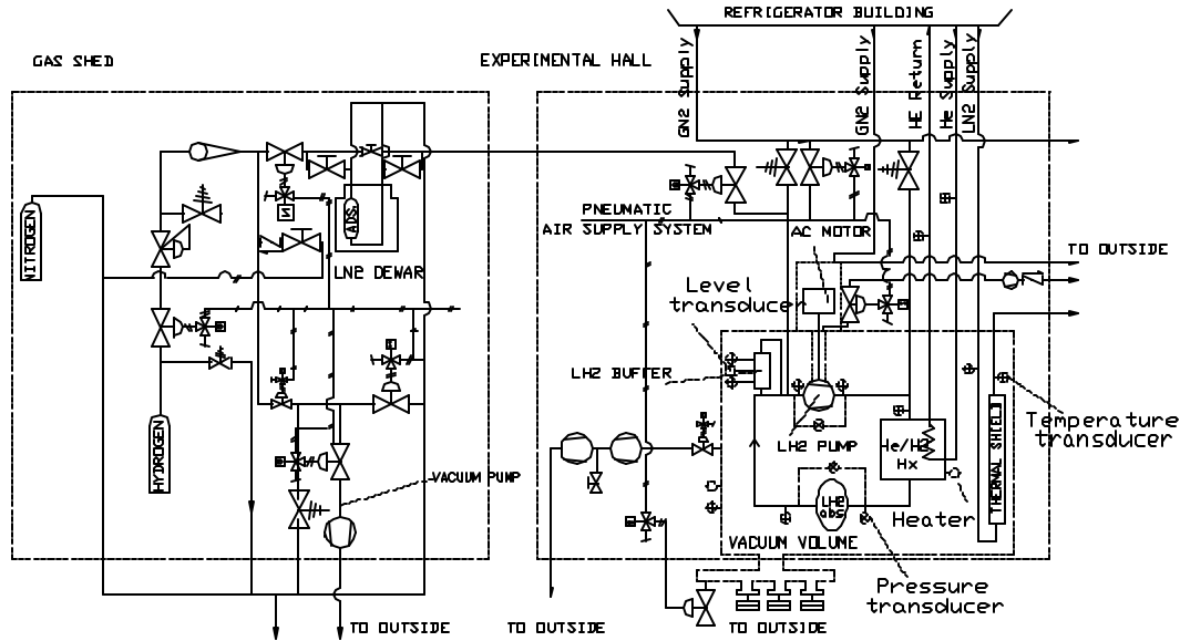
Figure 1: Flow schematic of the MuCool Test Area
