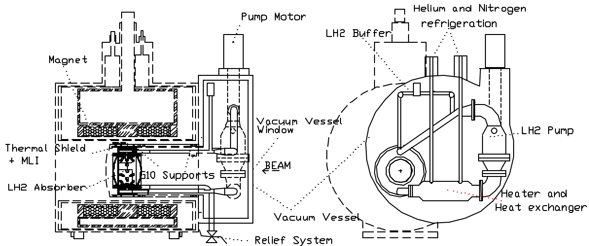
Figure 2: Conceptual design of the MuCool Test Area cryostat
