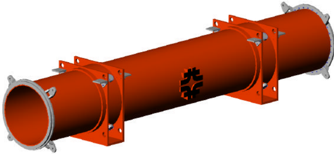
FIGURE 2. Vacuum vessel assembly.
