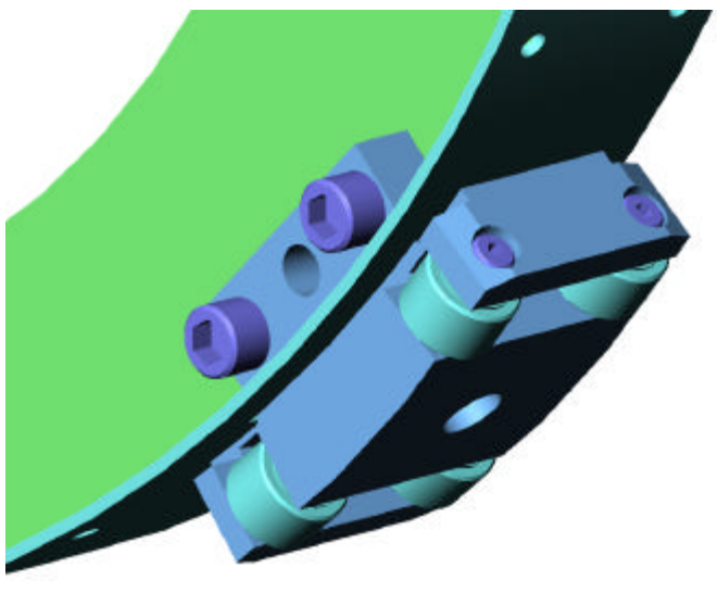
FIGURE 7. Close-up of support block and rollers.
