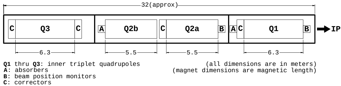
FIGURE 1. Schematic layout of a typical LHC interaction region inner triplet.
