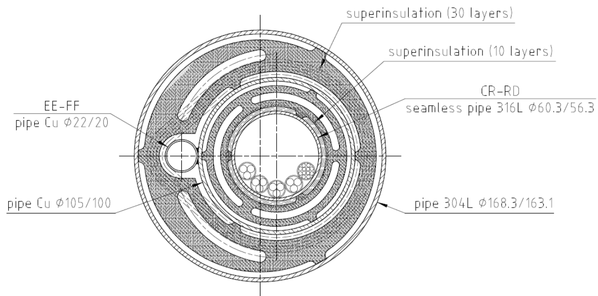
FIGURE 2. Type 1 DSL basic cross-section
