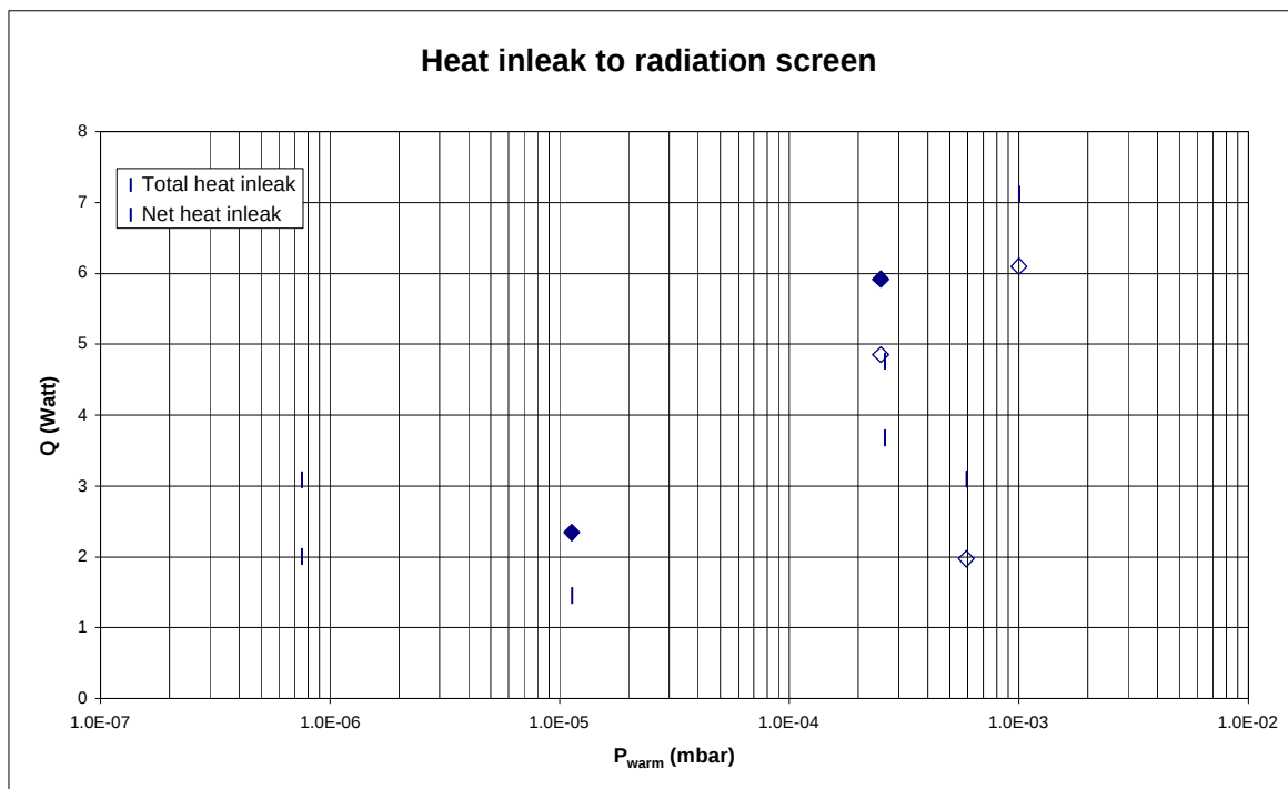
Figure 3.5: Total and net heat leak to the thermal shield with degraded vacuum conditions. P_{\text{warm}} is the pressure measured on the vacuum vessel wall, corrected for helium
