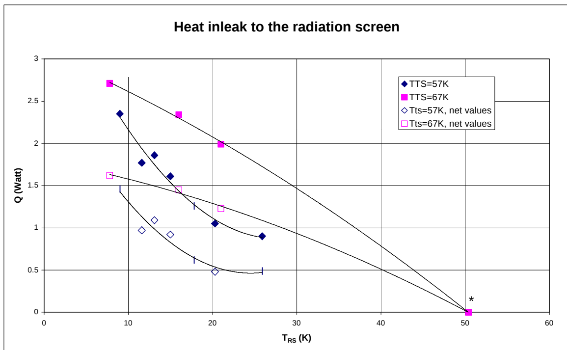
Figure 3.3: Total and net heat inleak to the radiation screen in CTM3 under degraded temperature conditions for the radiation screen, i.e. above 10 K, with a background helium pressure of 1.1 \cdot 10^{-5} mbar measured on the vacuum tank, and 1.6 \cdot 10^{-5} to 2 \cdot 10^{-5} mbar near the cold mass * no radiation screen cooling
